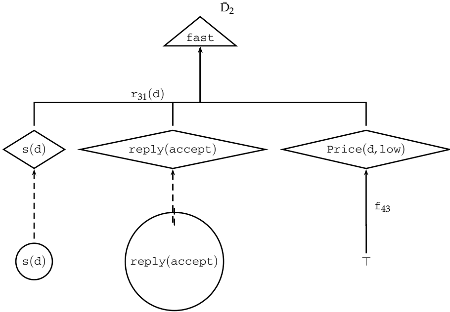
Fig. 1. The argument \bar{D}_2 concluding fast
