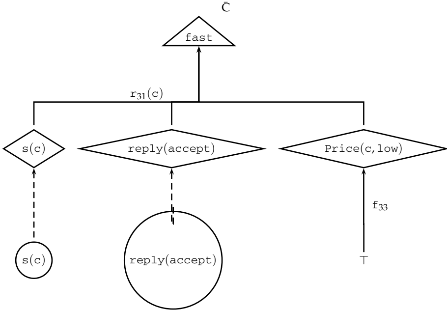
Fig. 2. The argument \bar{C} concluding fast
