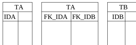
Figure F.10 – Projection d’une relation 1-n unidirectionnelle
