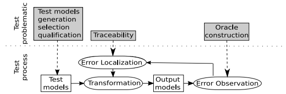
Figure 1: Test transformation process
