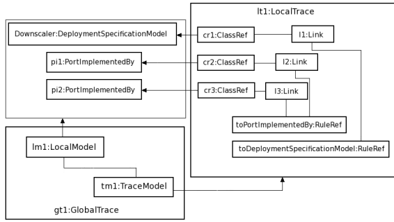
Figure 6: Excerpt of the output model, of the local and the global trace models
