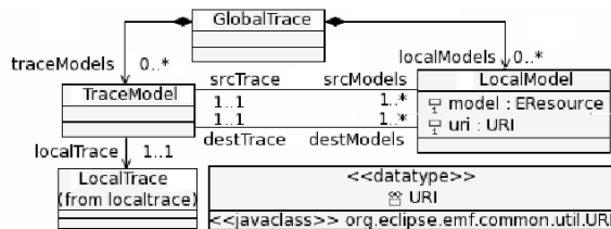
Figure 3: Global Trace Metamodel
